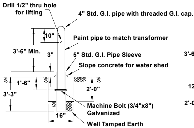
REMOVABLE BARRIER
